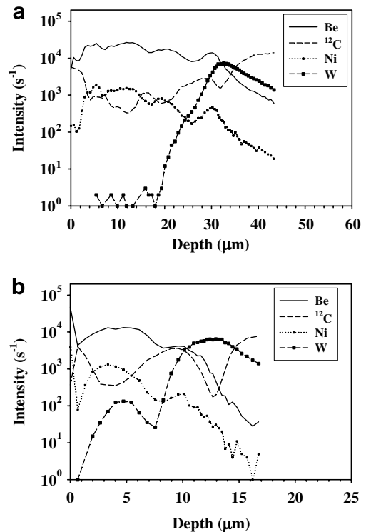
Fig. 2. SIMS depth profiles of Be, C, Ni and W from (a) from top of tile 1 (sample 1/8) and (b) from bottom of tile 1 (sample 1/2) (exposed in 2001–2004).
