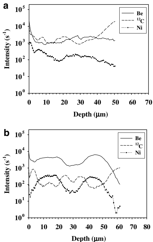
Fig. 3. SIMS depth profiles of Be, C and Ni from (a) from bottom of tile 3 (sample 3/2) and (b) from top of tile 3 (sample 3/8) (exposed in 1998–2004).
