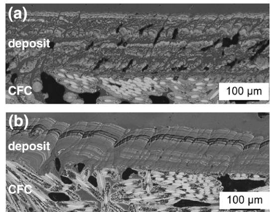
Fig. 6. Cross-sectional optical microscope image from sloping part of tile 4 (sample 4/7) (a) and from shadowed area (sample 4/9) (b).
