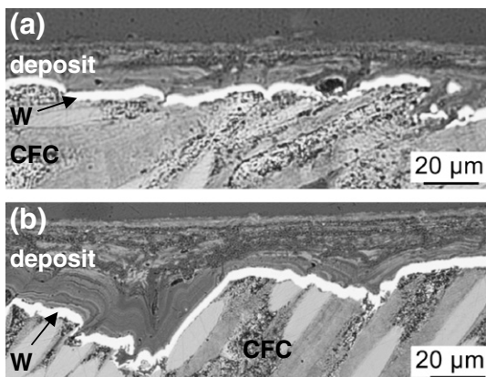
Fig. 4. Cross-sectional optical microscope image from bottom of tile 1 (sample 1/1) (a) and from top of tile 1 (sample 1/9) (b). Deposited film, W-marker layer and substrate marked in the figures.
