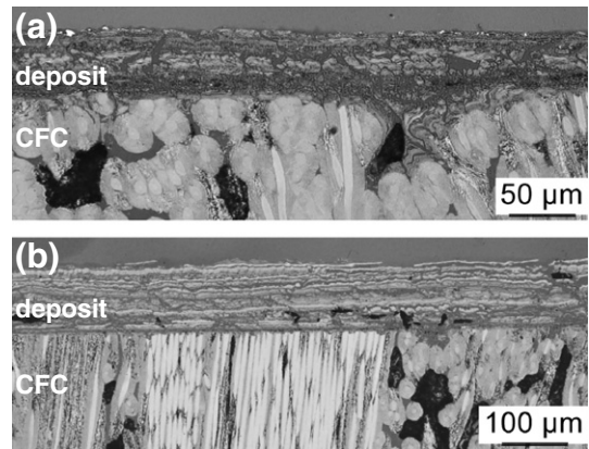
Fig. 5. Cross-sectional optical microscope image from bottom of tile 3 (sample 3/2) (a) and from top of tile 3 (sample 3/7) (b).
