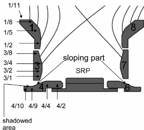
Fig. 1. The JET MkII-SRP divertor tile set. The samples for SIMS and IBA measurements are indicated with numbers. First number in the sample code refers to the tile and the second one to the poloidal location.
